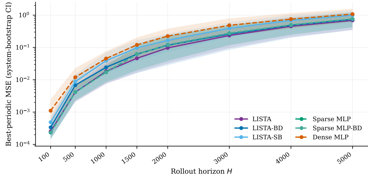
10-system Dysts forecasting performance
