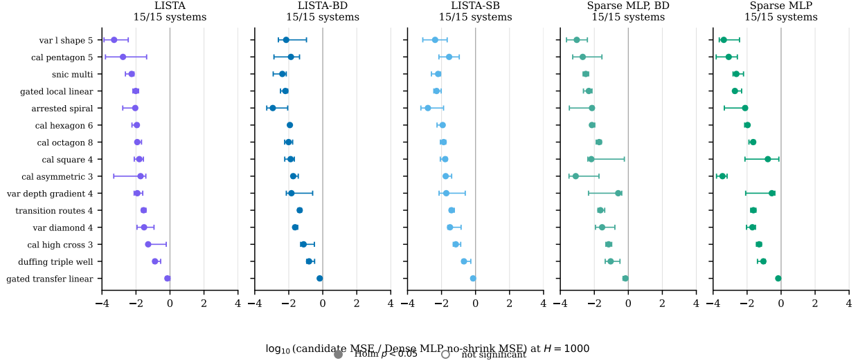
Figure 8: Per-system effect sizes at H=1000 versus the Dense MLP baseline. Each point is one benchmark system; the x -coordinate is the per-system median paired \log_{10} -MSE difference (candidate minus baseline) over the common completed seeds, up to 15 per system, with whiskers showing the 95% bootstrap interval. Filled markers clear Holm-corrected \alpha=0.05 . Numerical values are in table 9 .
