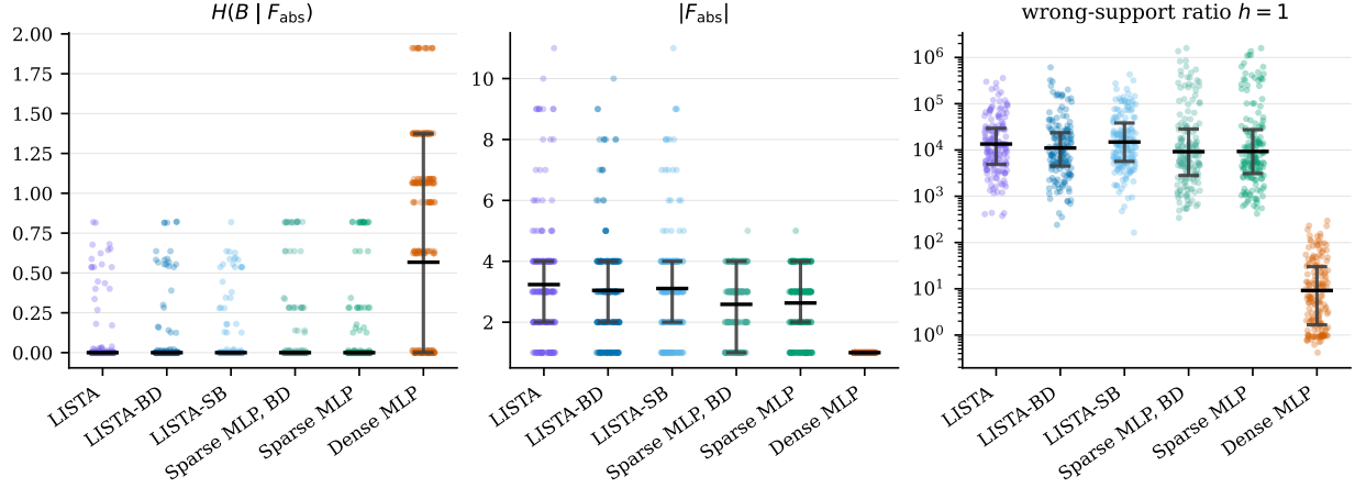
Figure 2: Per-seed support results on the deep-state slice. Dots show system–seed pairs, and gray I-bars mark first-to-third quartile ranges. Black bars mark the paper-facing summary: seed-IQM within each system followed by an arithmetic mean across systems for entropy and wrong-support ratios, and arithmetic means for |F_{\text{abs}}| . Lower is better for H(B | F_{\text{abs}}) ; |F_{\text{abs}}| is a non-directional support-family count to compare with the represented basin count. The wrong-support panel shows wrong-support/base ratios at h=1 on a log scale; higher means that using a wrong-basin support is more damaging.
