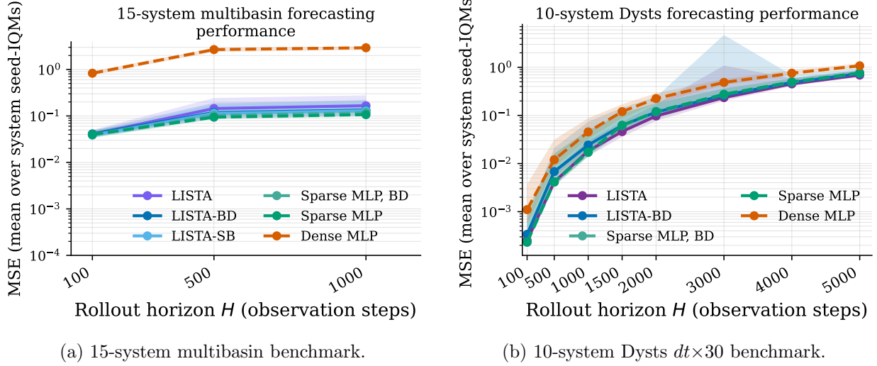
Figure 3: Forecasting horizon trends. Lines show arithmetic means across per-system seed-IQM MSEs on a log scale, and bands show fixed-system seed-bootstrap 95% intervals for the same estimand.
