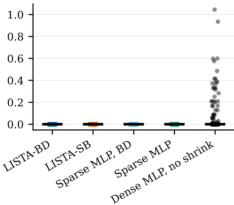
H(B|S) deep
