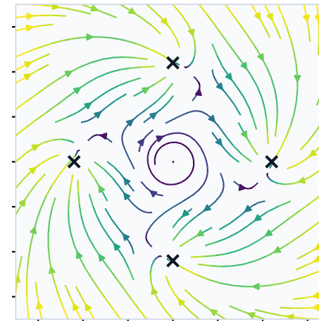
14. Diamond four-well
