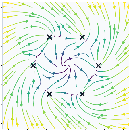
11. SNIC multi-attractor
