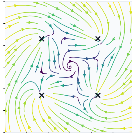
13. Depth-gradient four-well
