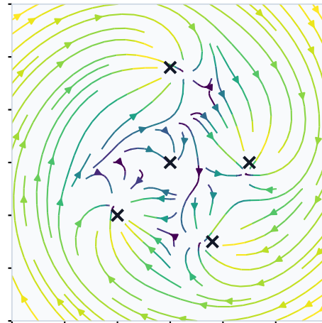
8. Pentagonal five-well
