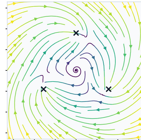
10. Triple-well Duffing
