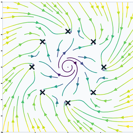
12. Transition-routes four-well
