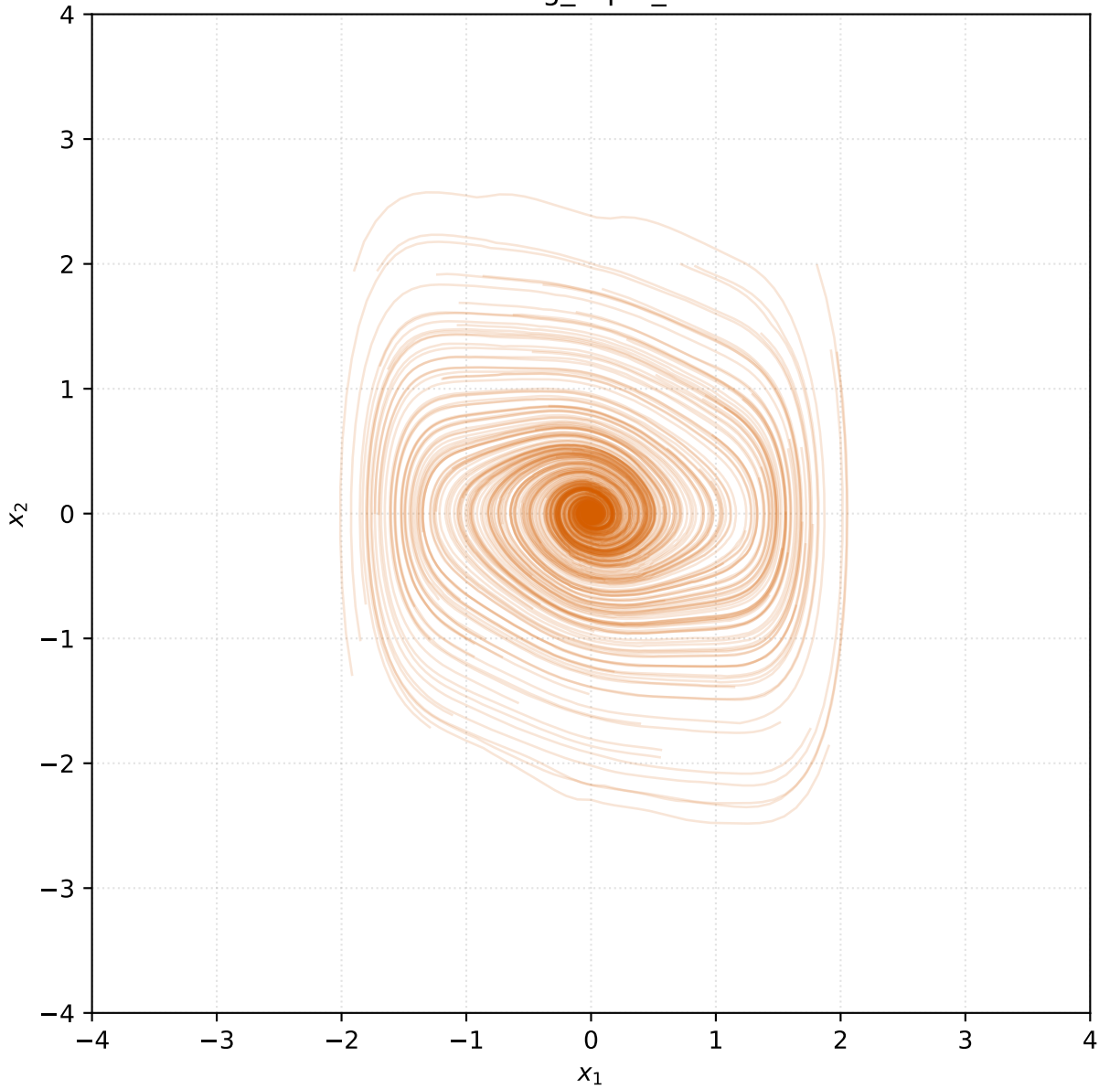
duffing_triple_well
