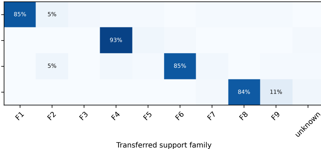
Temporal sparse KAE, all trajectories (9 families + unknown)
