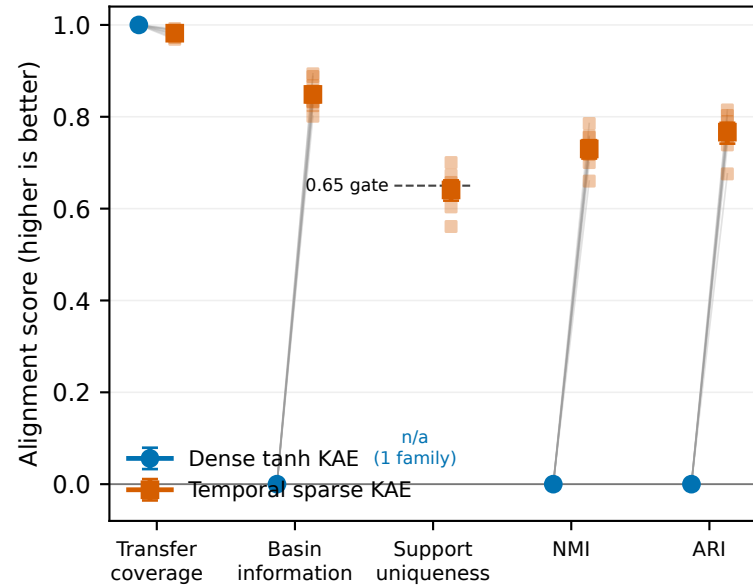
c Transferred PDE basin-support alignment
