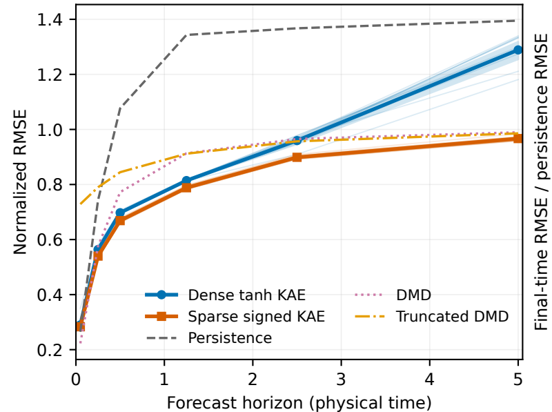
a Chaotic forecasting: Lorenz-96 ( d_x = 128 )
