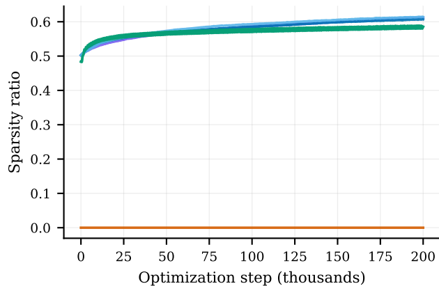
Sparsity-ratio diagnostic
