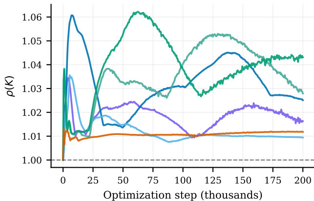
Spectral radius of K
