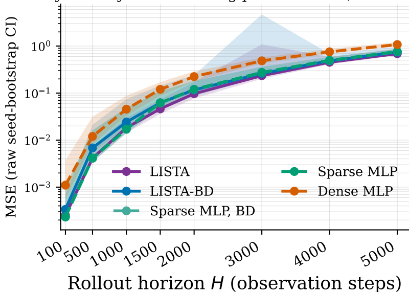
10-system Dysts forecasting performance (raw seed CI)
