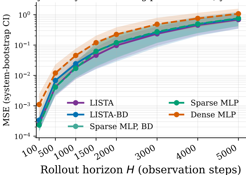
10-system Dysts forecasting performance (system CI)
