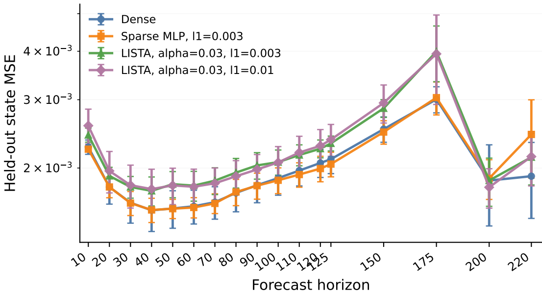
ManiSkill perturbation forecasting (best periodic)
