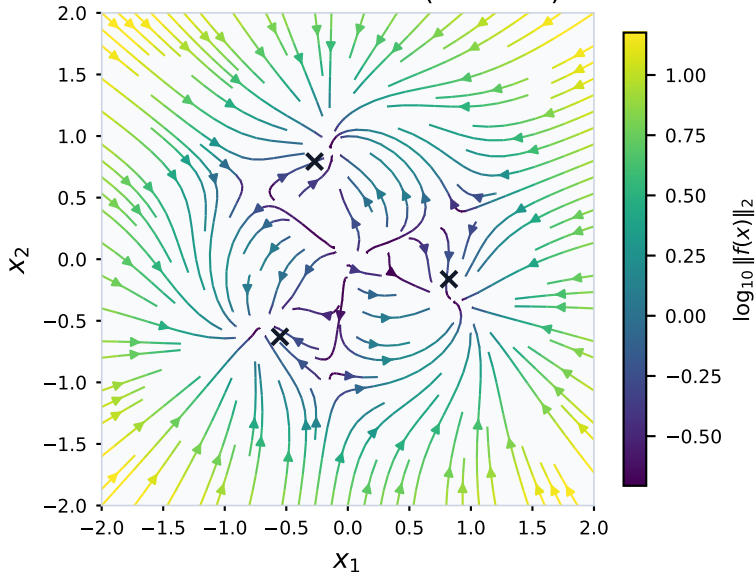
SNIC multi-attractor (3 basins)
