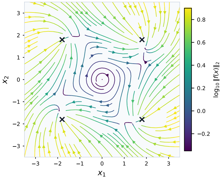
Transition-routes four-well (4 basins)
