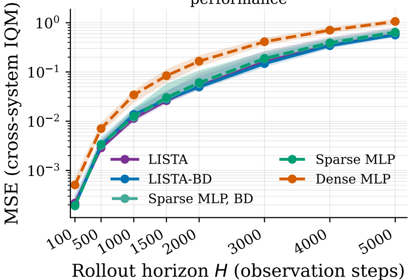
12-system Dysts forecasting performance
