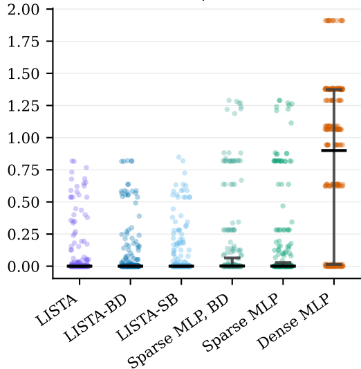
H(B | F_{\text{abs}})
