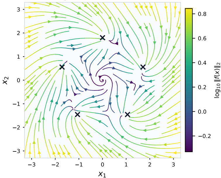
Pentagonal five-well (5 basins)
