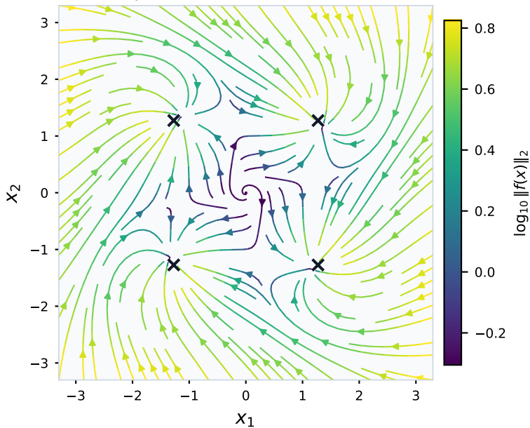
Square four-well (4 basins)
