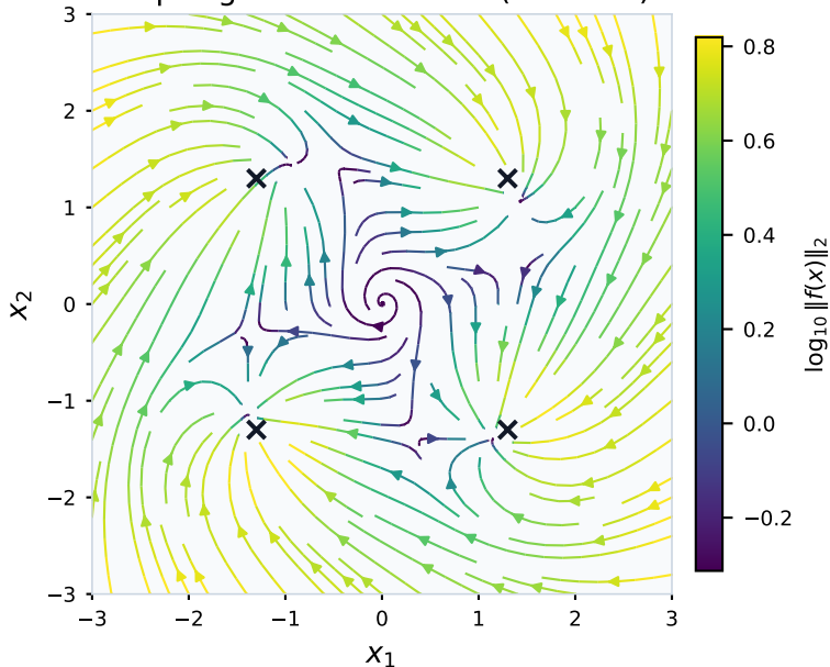
Depth-gradient four-well (4 basins)
