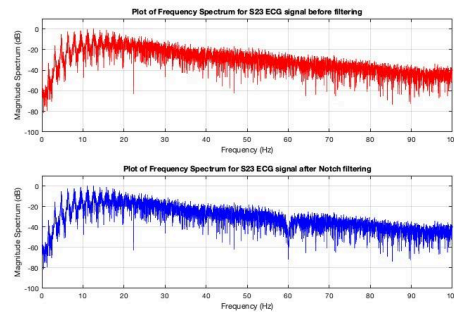
Figure 5: The frequency spectrum of the ECG signal for Subject 23's diabetic signal shows the before-and-after plots following notch filtering.
