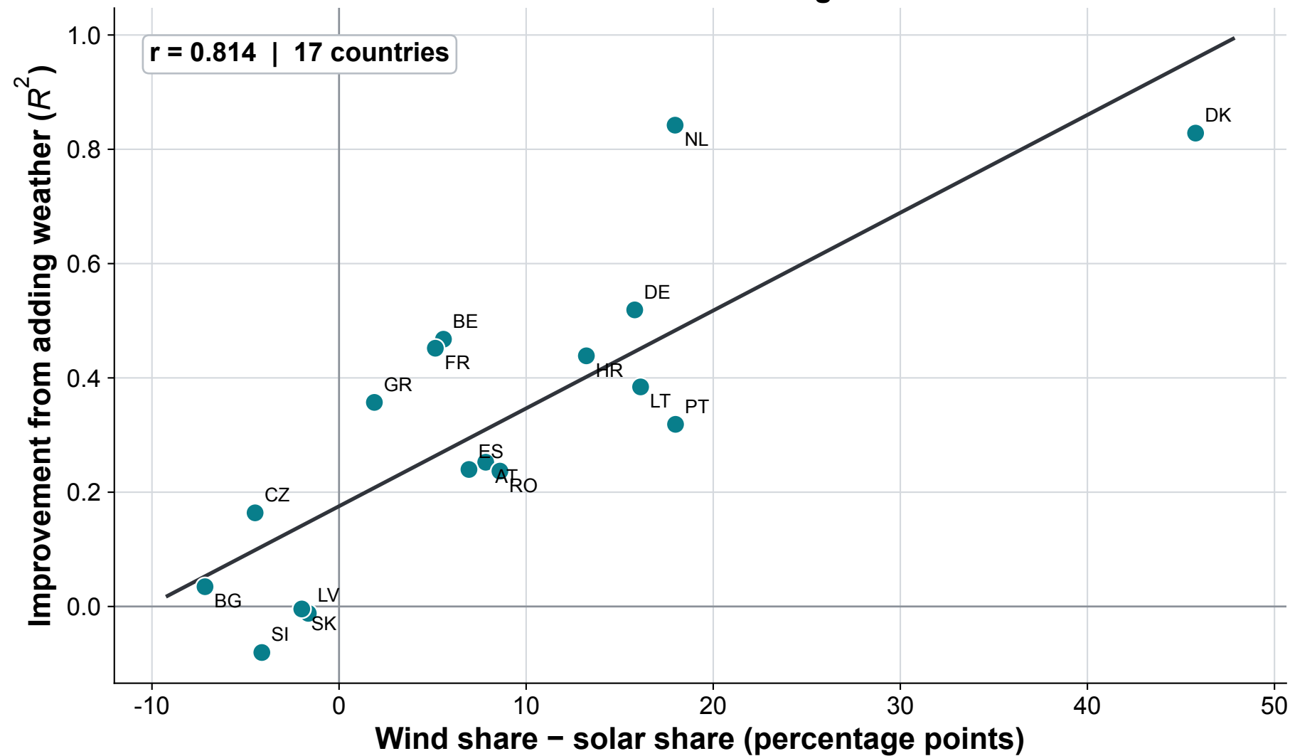
Gradient Boosting
