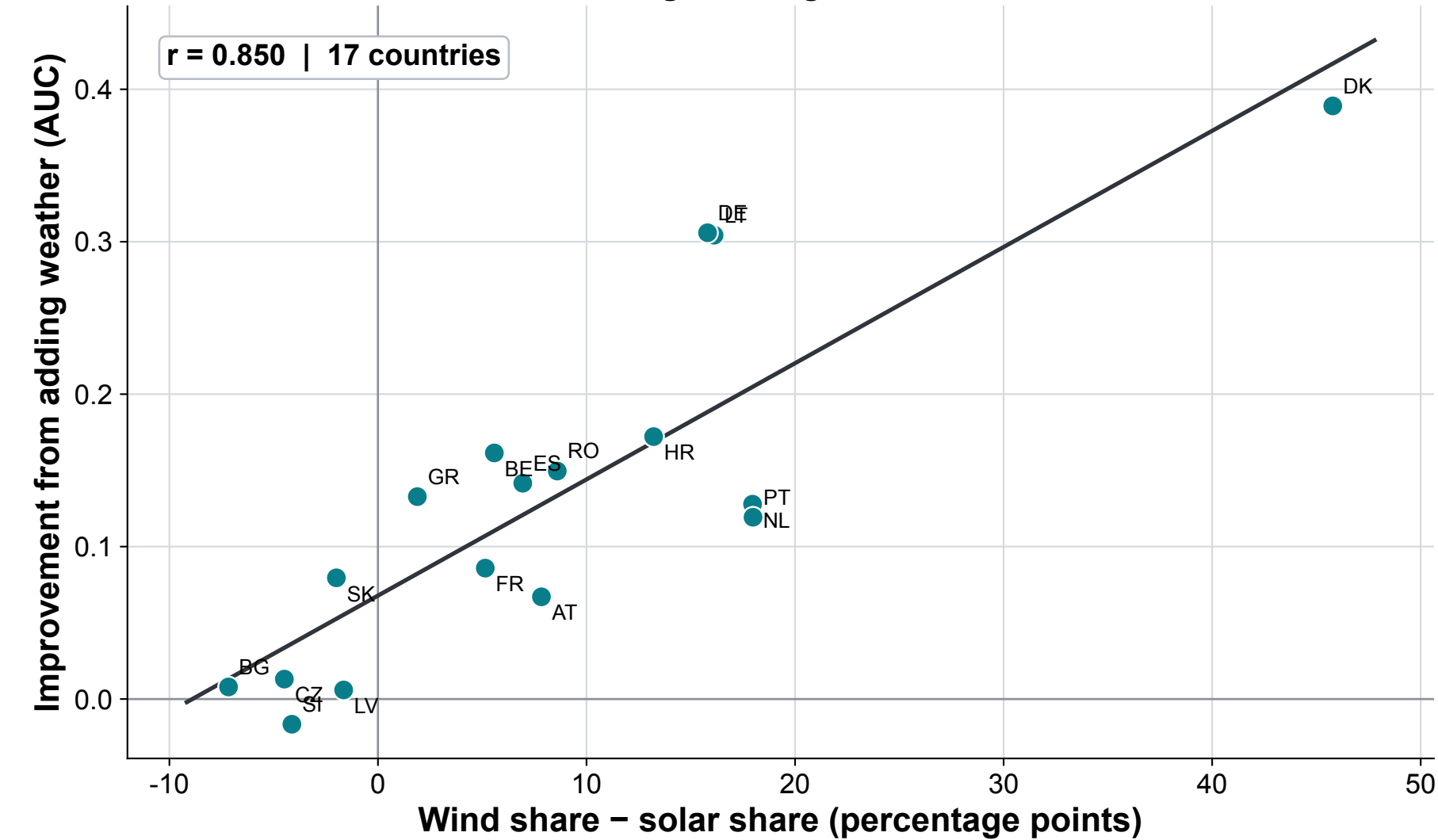
Gradient Boosting
