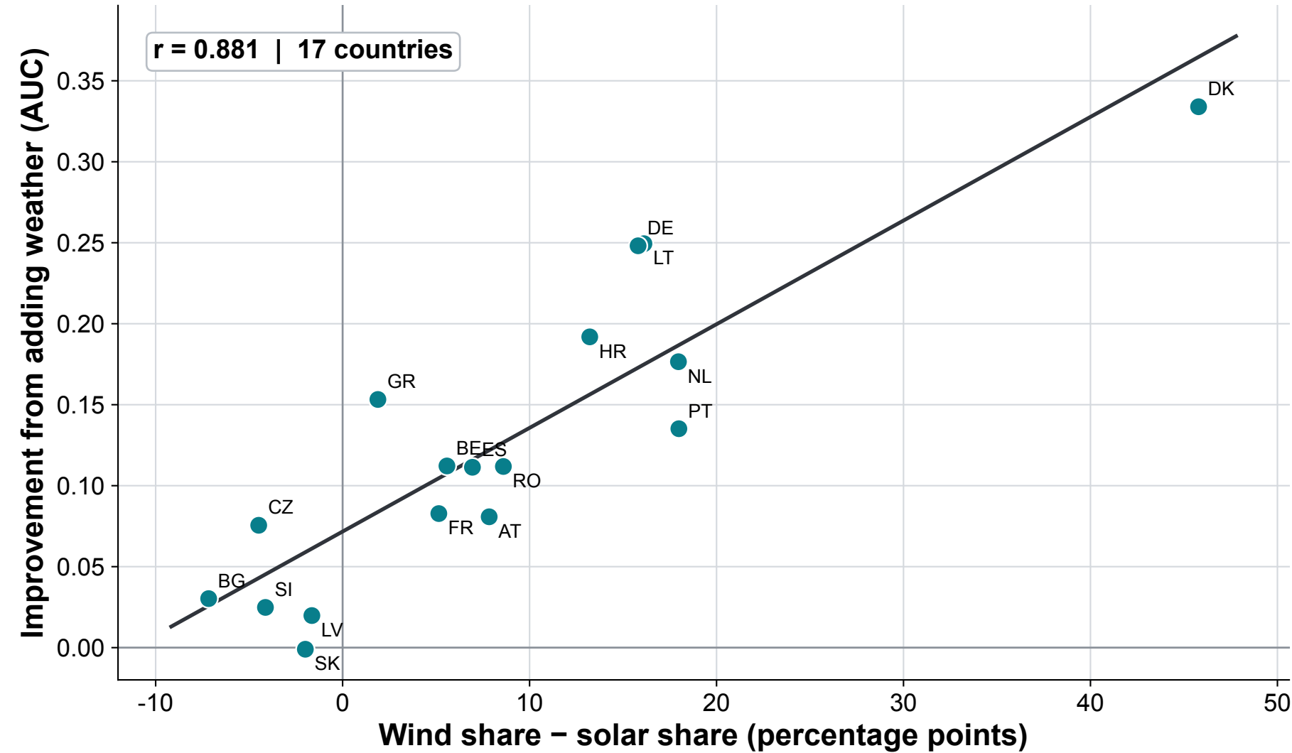
LightGBM
