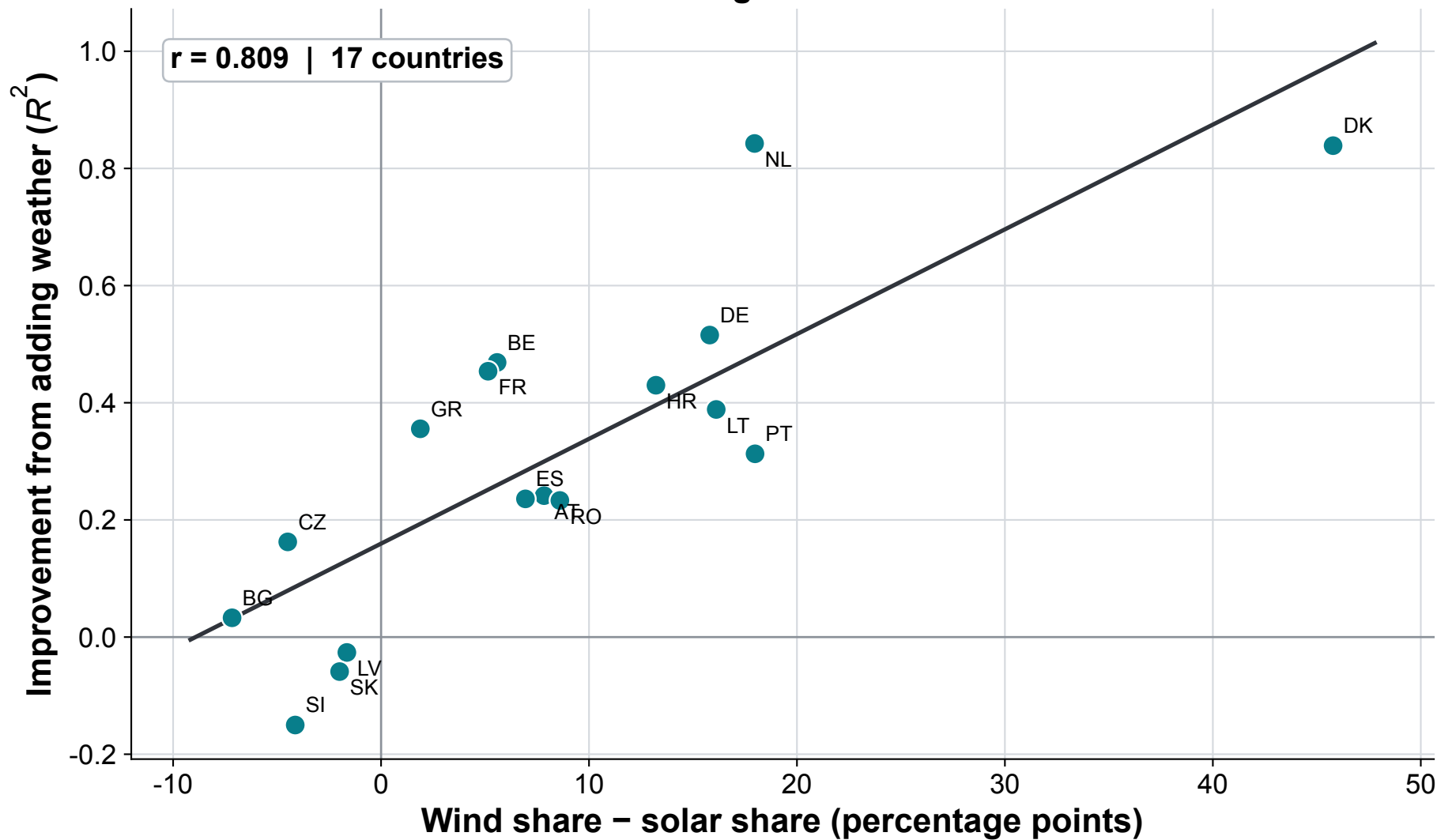
LightGBM
