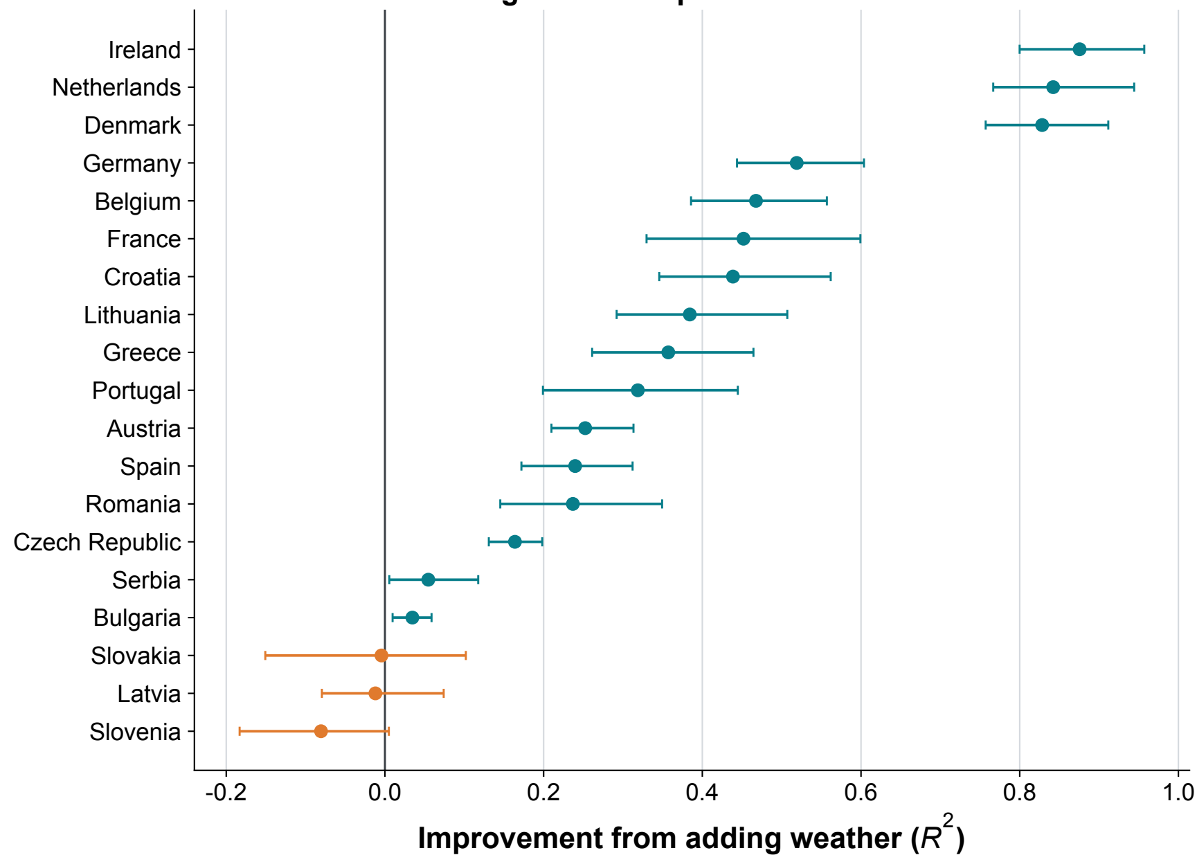
Gradient Boosting — clear improvement in 16 of 19 countries
