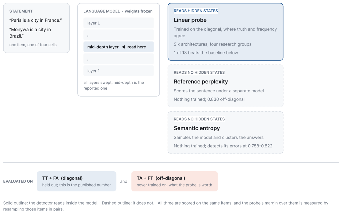
Figure 5: What each detector is allowed to read. The probe taps one layer of a frozen model and is trained on the diagonal; the two comparators never open the model at all. All three are scored on the same items, and the probe’s margin over them is measured by resampling those items in pairs. Solid outline marks a detector that reads inside the model, dashed one that does not.
