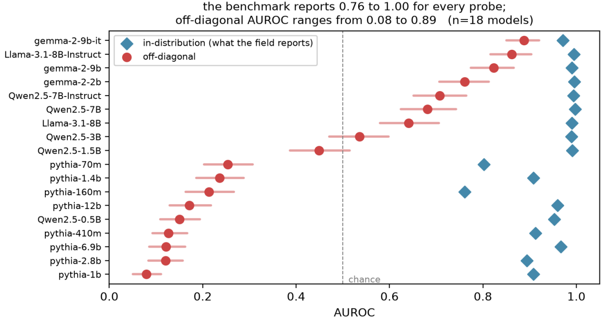
Figure 3: The benchmark reports 0.76 to 1.00 for every probe; off-diagonal AUROC ranges from 0.08 to 0.89
