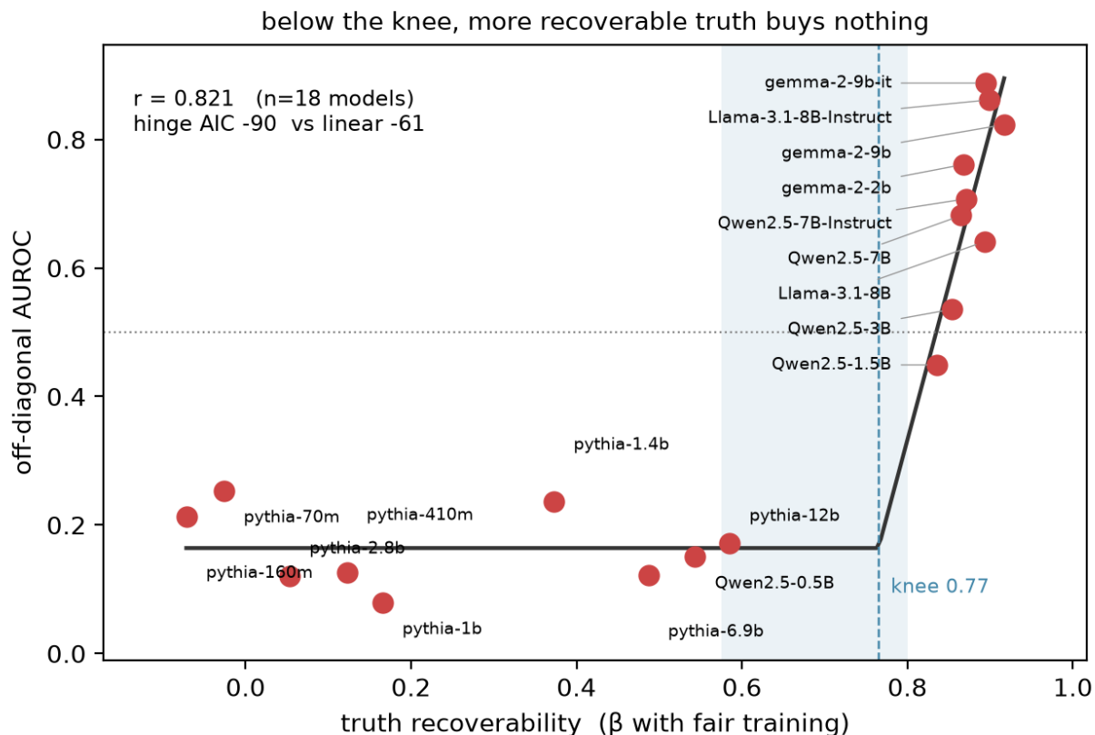
Figure 4: Below the knee, more recoverable truth buys nothing
