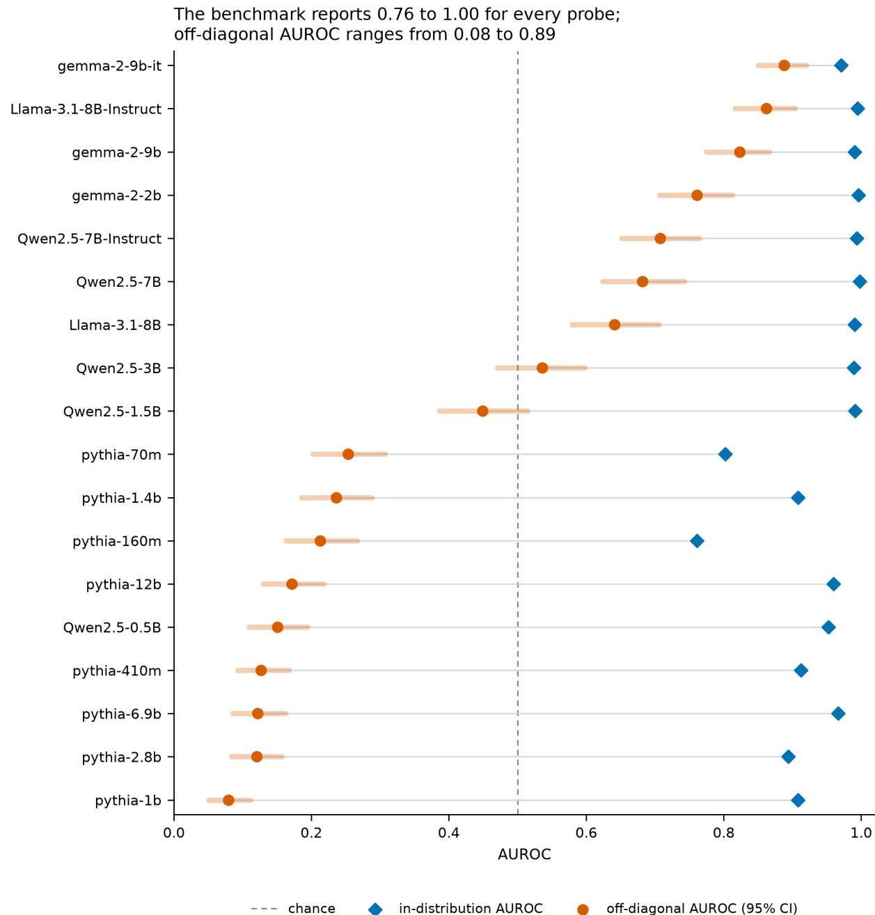
Figure 3: Every probe scores 0.76 to 1.00 on the split the field reports (diamond, in-distribution AUROC) and 0.08 to 0.89 once truth and entity frequency are pulled apart (circle, off-diagonal AUROC with its 95% bootstrap interval). Models are ordered by off-diagonal AUROC.
