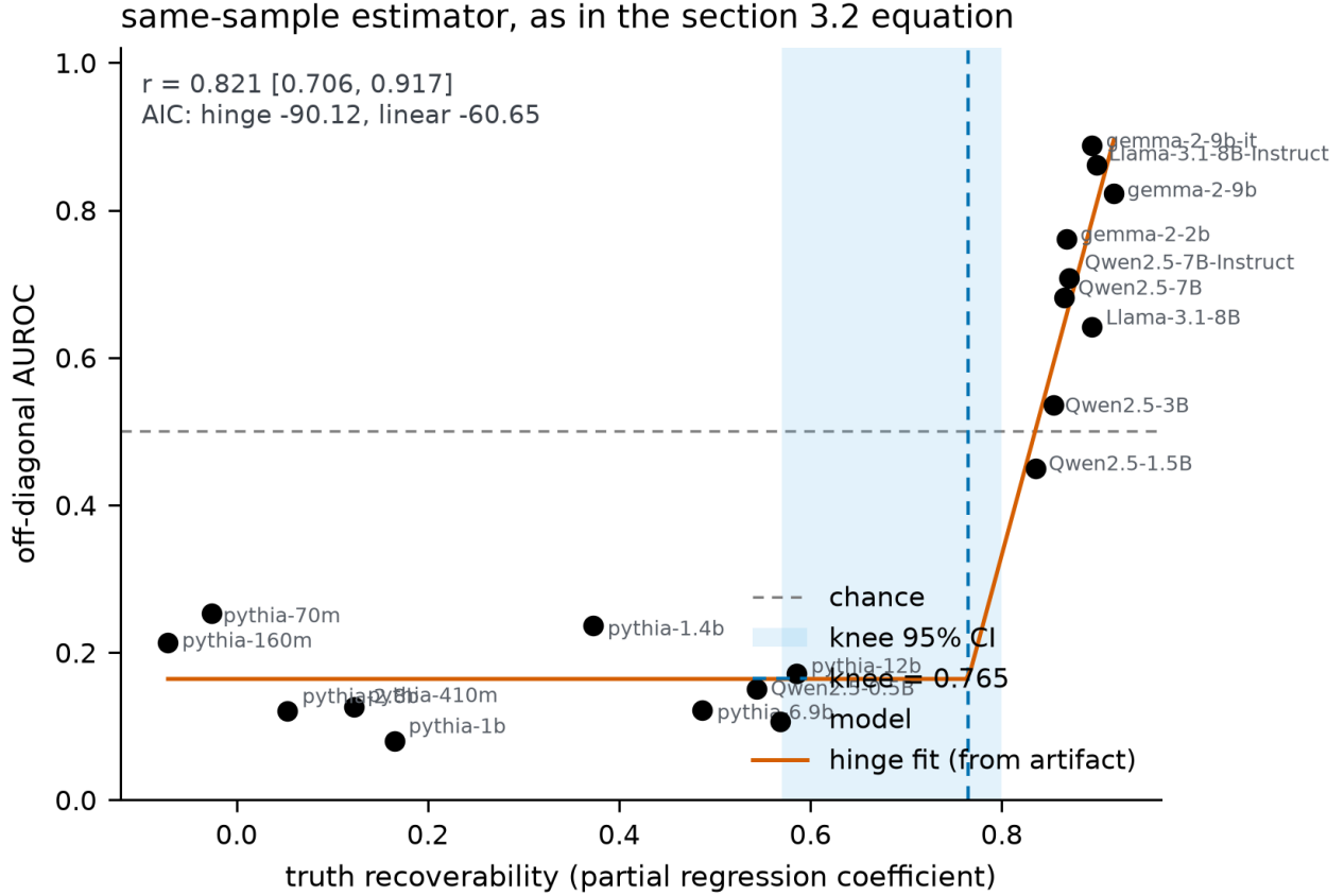
Figure 5: Off-diagonal AUROC against truth recoverability, one point per model. The hinge is the fit stored in the artifact, not refitted here; the shaded band is the knee’s 95% bootstrap interval. Below the knee, additional recoverability buys nothing.
