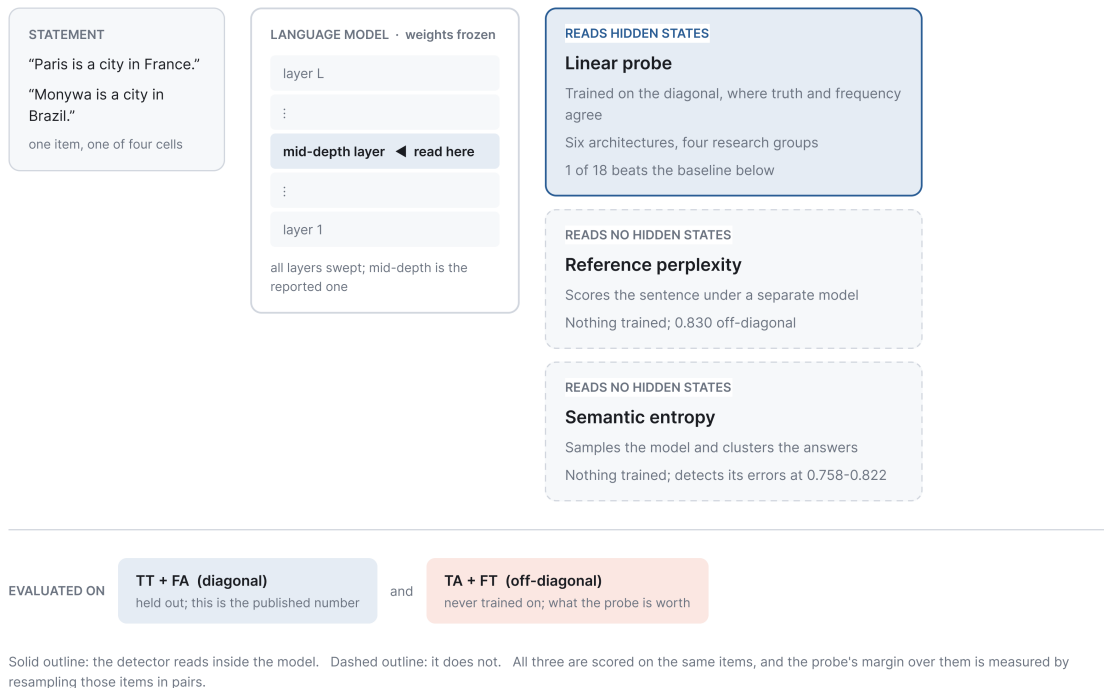
Figure 7: What each detector is allowed to read. The probe taps one layer of a frozen model and is trained on the diagonal; the two comparators never open the model at all. All three are scored on the same items, and the probe’s margin over them is measured by resampling those items in pairs. Solid outline marks a detector that reads inside the model, dashed one that does not.
