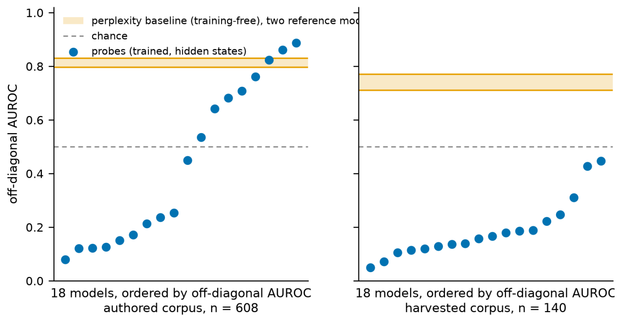
Figure 8: Off-diagonal AUROC for every probe against the training-free perplexity baseline, one panel per corpus. The band spans the two reference models. On the harvested corpus every probe sits below it.
