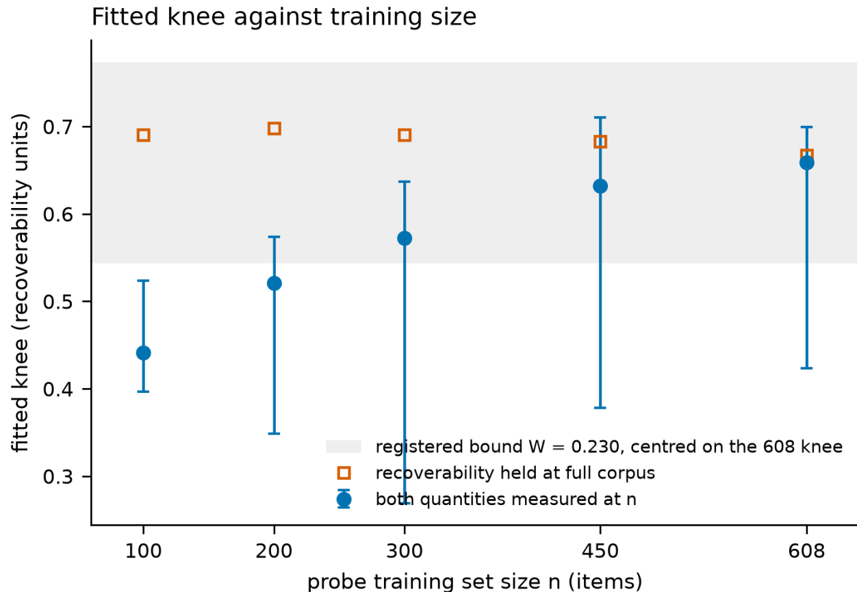
Figure 6: Fitted knee against probe training size, both registered designs, with the bound fixed in advance. Points and intervals only: the registered test returned indeterminate, so no trend is drawn.
