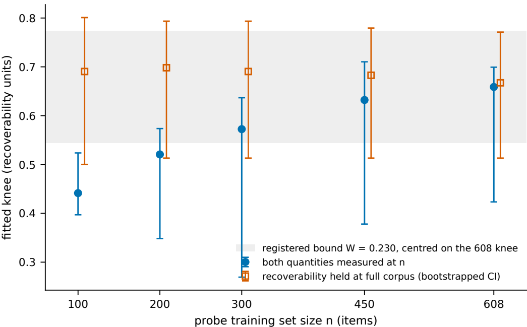
Fitted knee against training size
