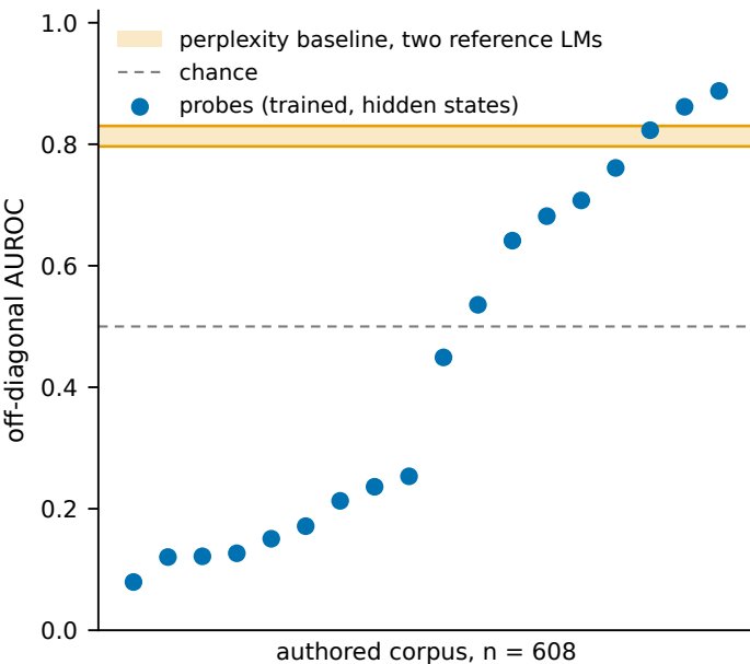
Probes against a detector that reads no hidden states 18 models per panel, ordered by off-diagonal AUROC
