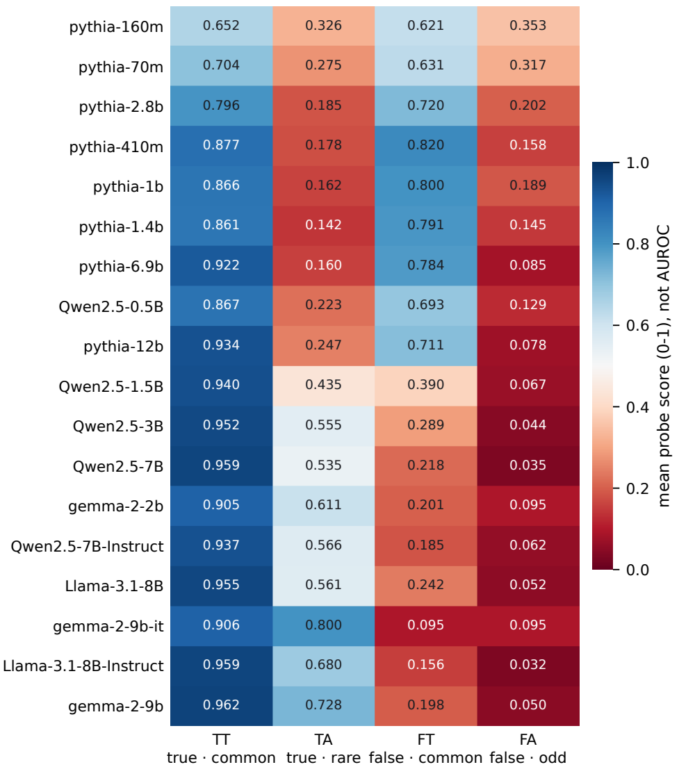
Mean probe score by cell, models ordered by recoverability
