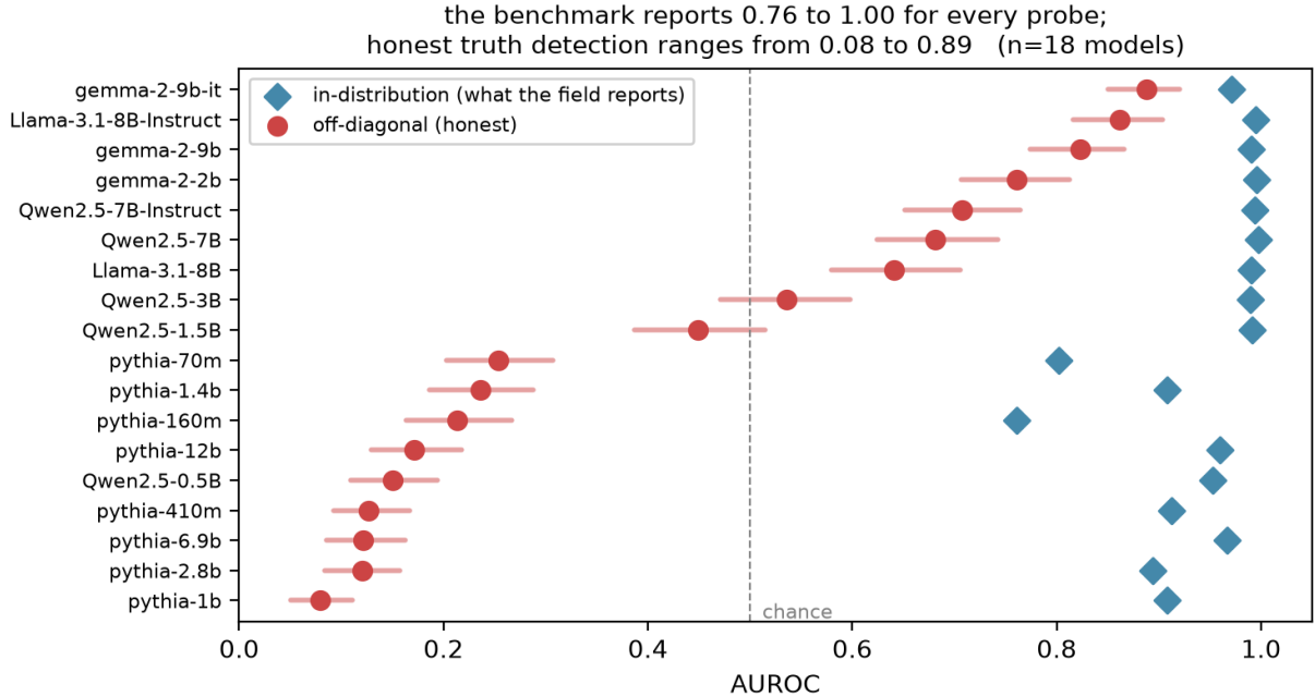
Figure 2: The benchmark reports 0.76 to 1.00 for every probe; off-diagonal AUROC ranges from 0.08 to 0.89
