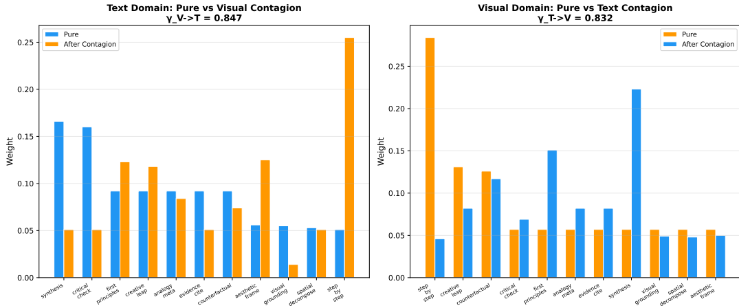
Figure 3: Strategy inversion before and after cross-modal contagion. Optimal strategies swap between modalities.
