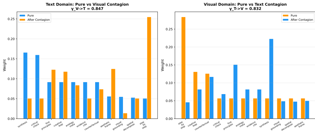
Figure 3: Strategy inversion before and after cross-modal contagion. Optimal strategies swap between modalities.
