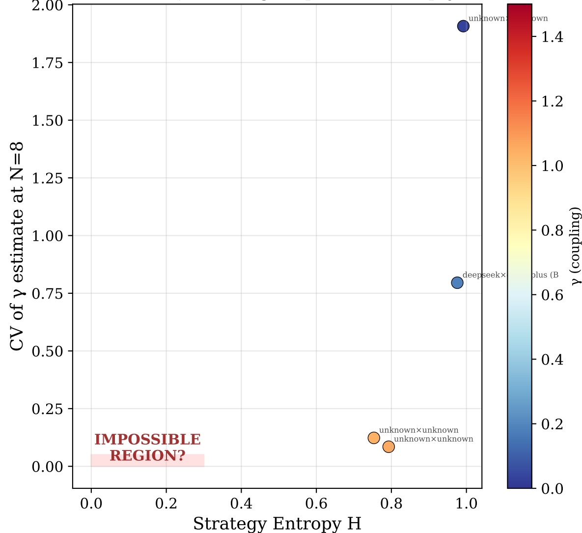
C. The Triangle: H vs. CV(N=8) Color = \gamma , Red region predicted empty
