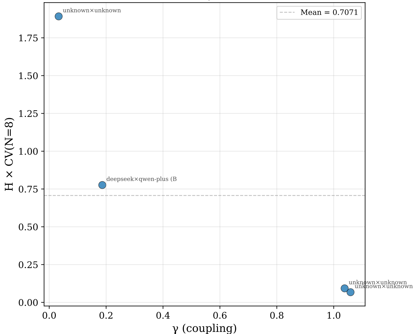
D. H × CV product vs. \gamma Bounded away from zero?
