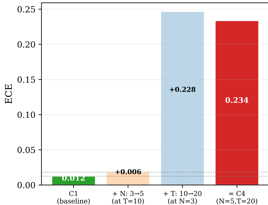
Factor Effect Decomposition
