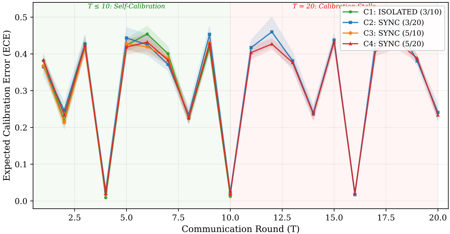
Calibration Contagion: ECE Trajectories Across Conditions
