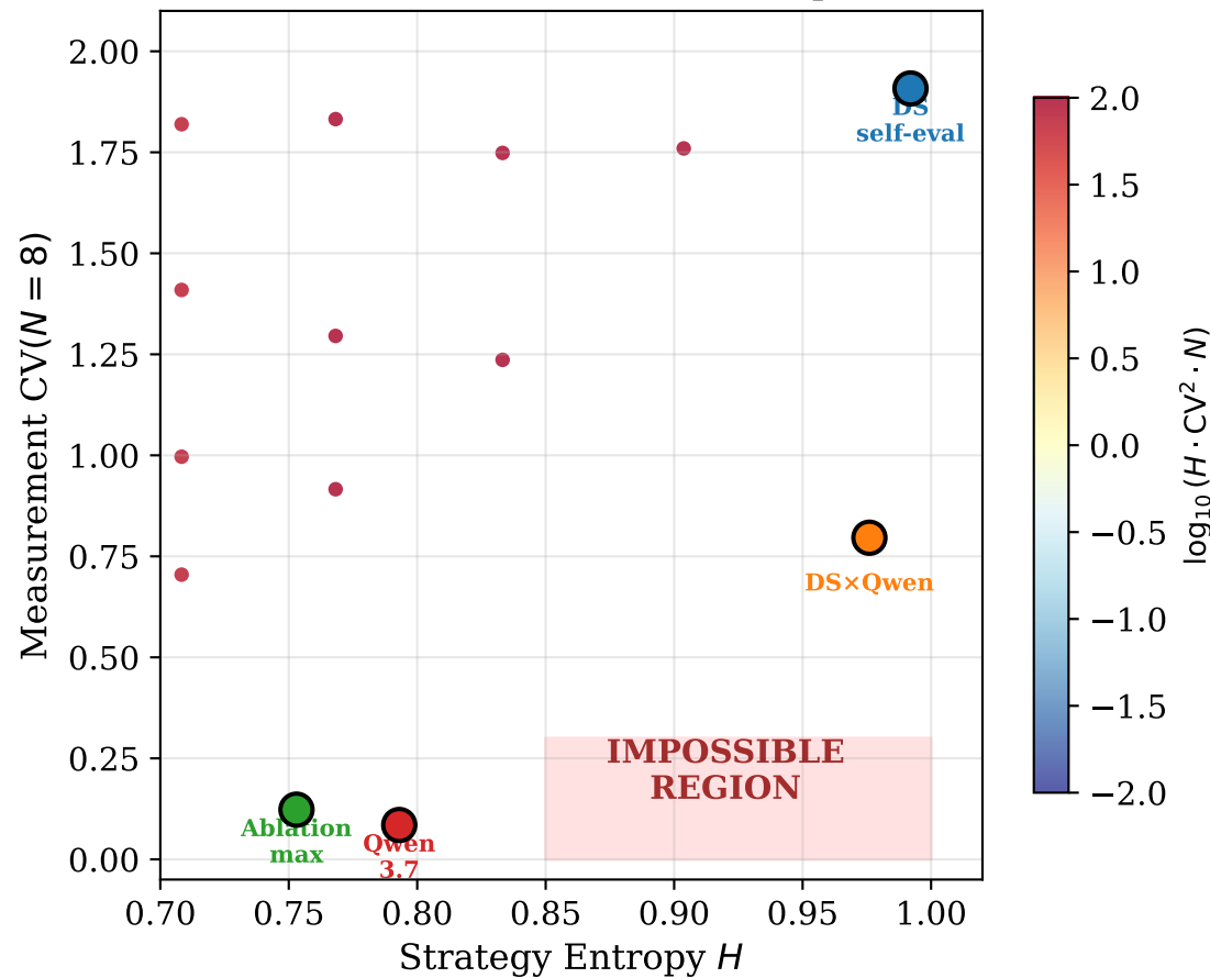
A. Phase Diagram: H vs. CV (Color = H \cdot CV^2 \cdot N ; White = low product)
