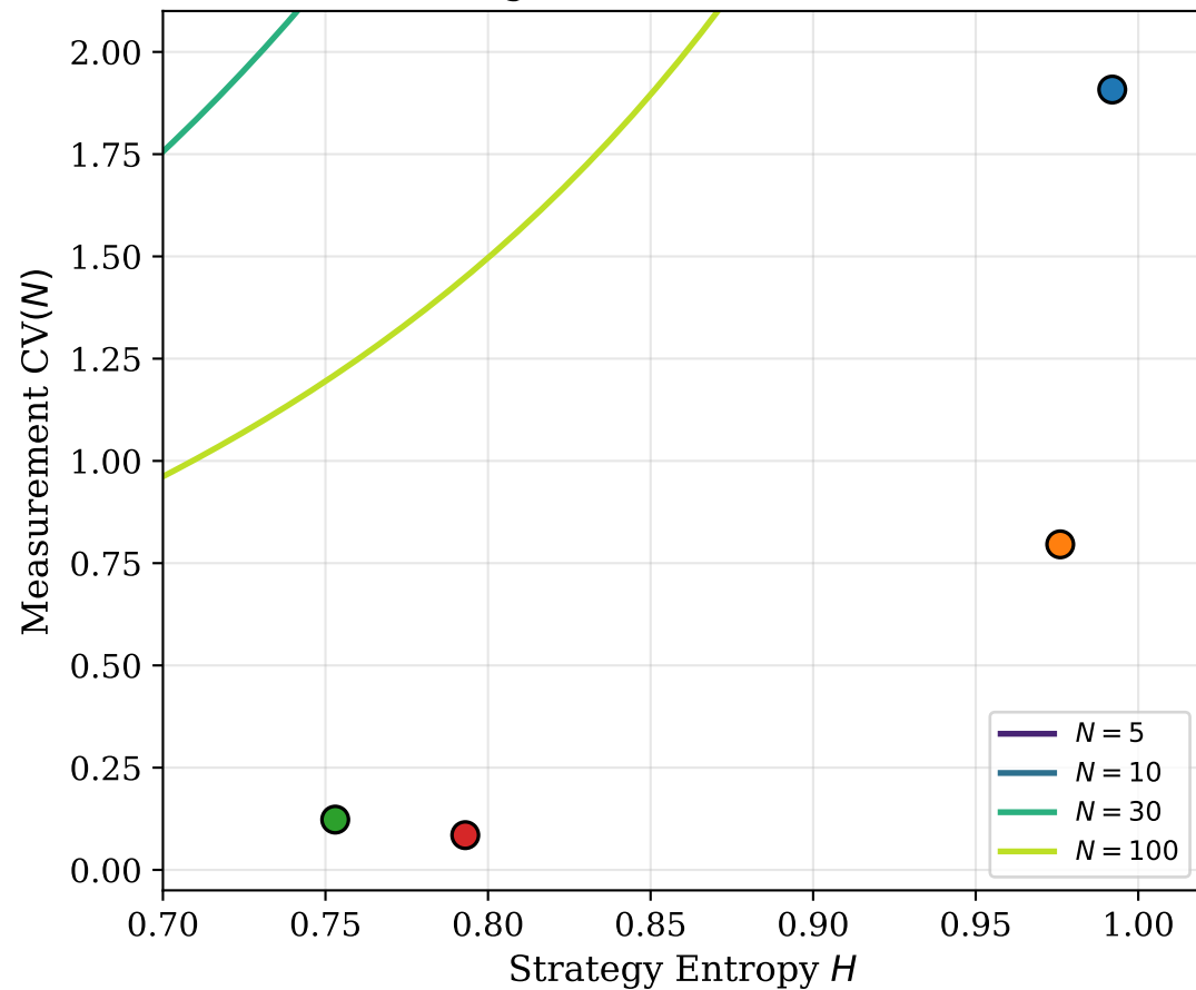
B. Trade-off Curves at Fixed N (Increasing N shifts curves downward)
