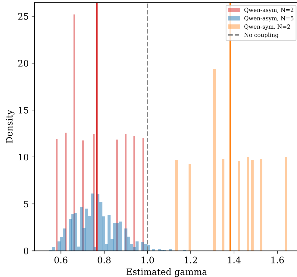
B. N-Sensitivity in Qwen P(g < 1 | N=2) = 100\% , P(g < 1 | N=5) = 98\%
