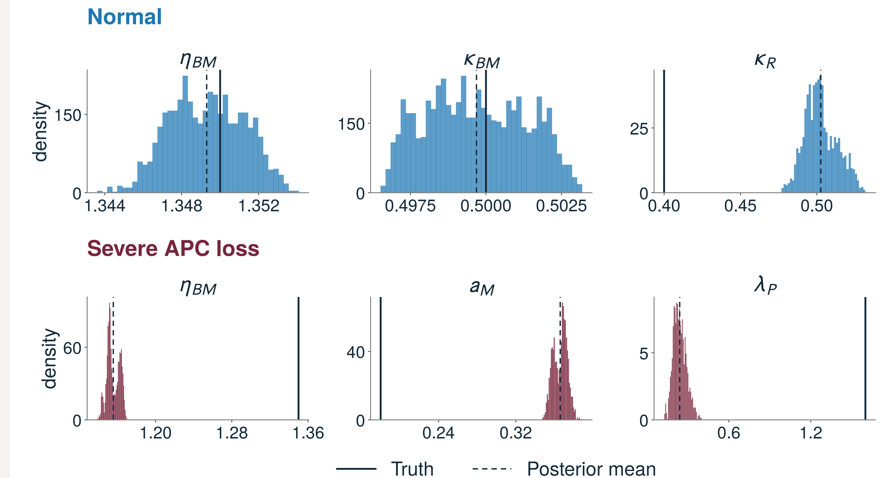
Fig. 6. Presentation marginals (2000 draws/regime): narrow distributions can miss truth.
