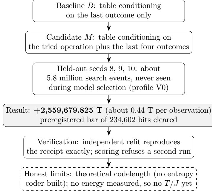
Figure 2: Schematic of the recorded first canonical Turing measurement (2026-09-29, profile V0, omega PR 85). This diagram restates the reported run; it is a schematic of a recorded measurement, not new data.
