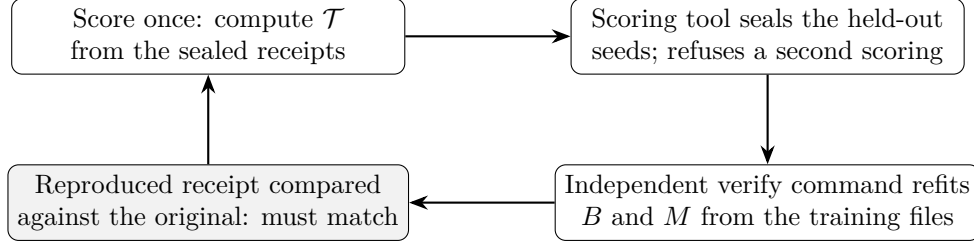
Figure 3: Conceptual schematic of the verification-by-refit loop used for the first canonical measurement (Section 7). The held-out data can be scored exactly once; reproducibility is established by refitting both models from the training files and reproducing the receipt bit for bit. Conceptual illustration, not empirical data.
