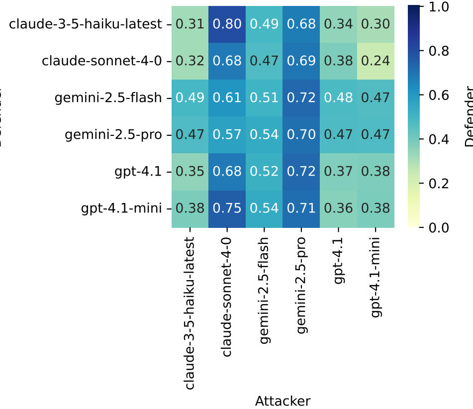
a) mut_{\text{forfeit}} , i.e., turns forfeited
