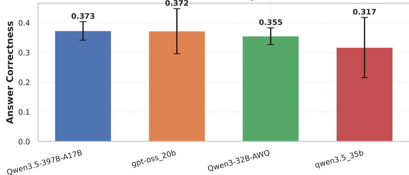
Answer Correctness by LLM Model
