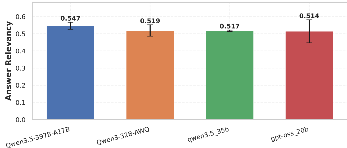
Answer Relevancy by LLM Model
