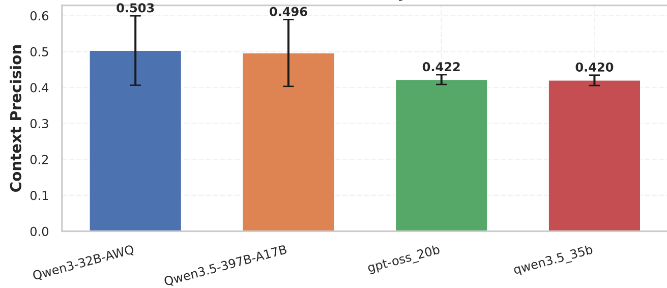
Context Precision by LLM Model
