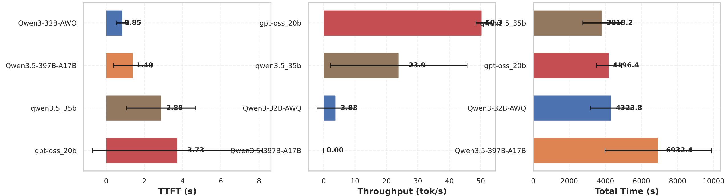
TTFT (s) (lower is better)
