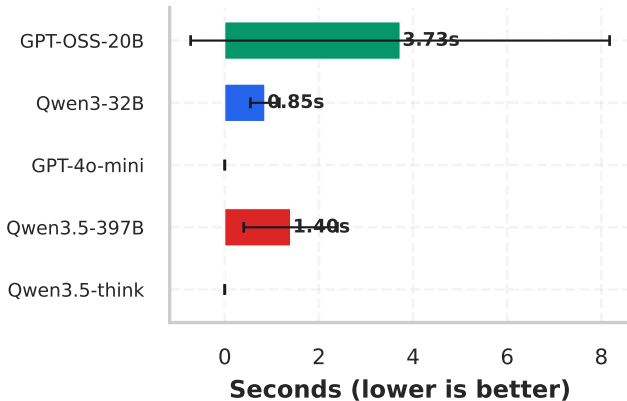
Time to First Token
