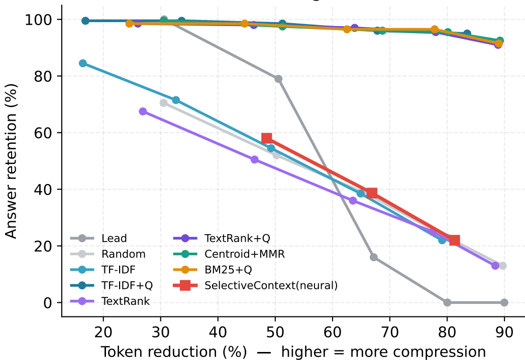
Answer retention vs. compression (multi-doc SQuAD, gold in middle)
