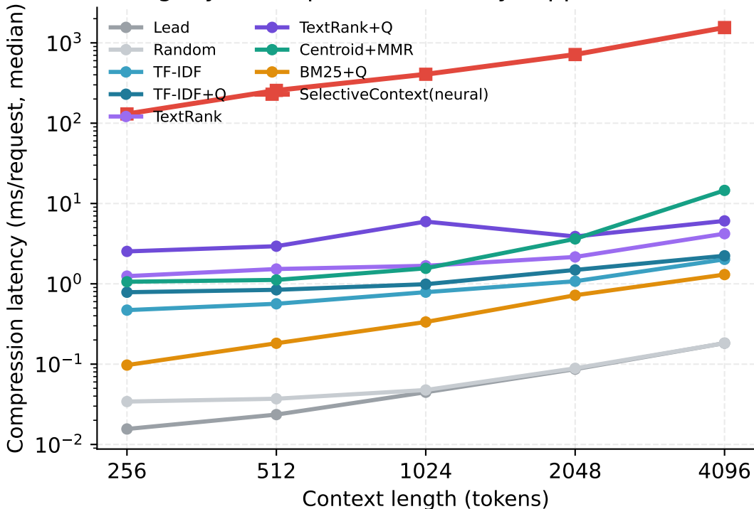
Routing-layer compression latency (Apple M3 Pro, CPU)
