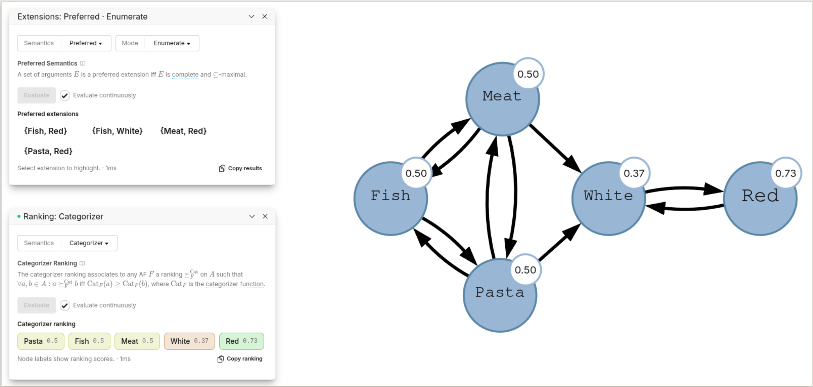
Preferred extensions enumerated; the categoriser ranking annotated on each argument.
