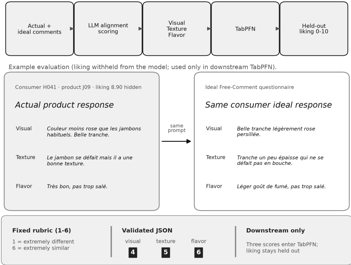
Figure 1: Direct LLM alignment scoring. Top: pipeline from paired Free-Comment text to held-out liking. Bottom: example evaluation (liking withheld from the model) with fixed 1-6 rubric, validated JSON scores, and TabPFN inputs.
