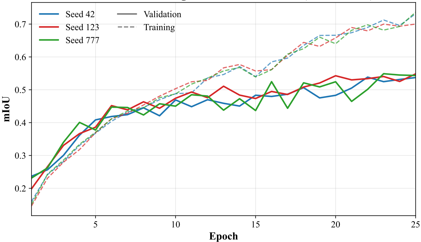
ERP-CBAM Training and Validation mIoU (Three Seeds)
