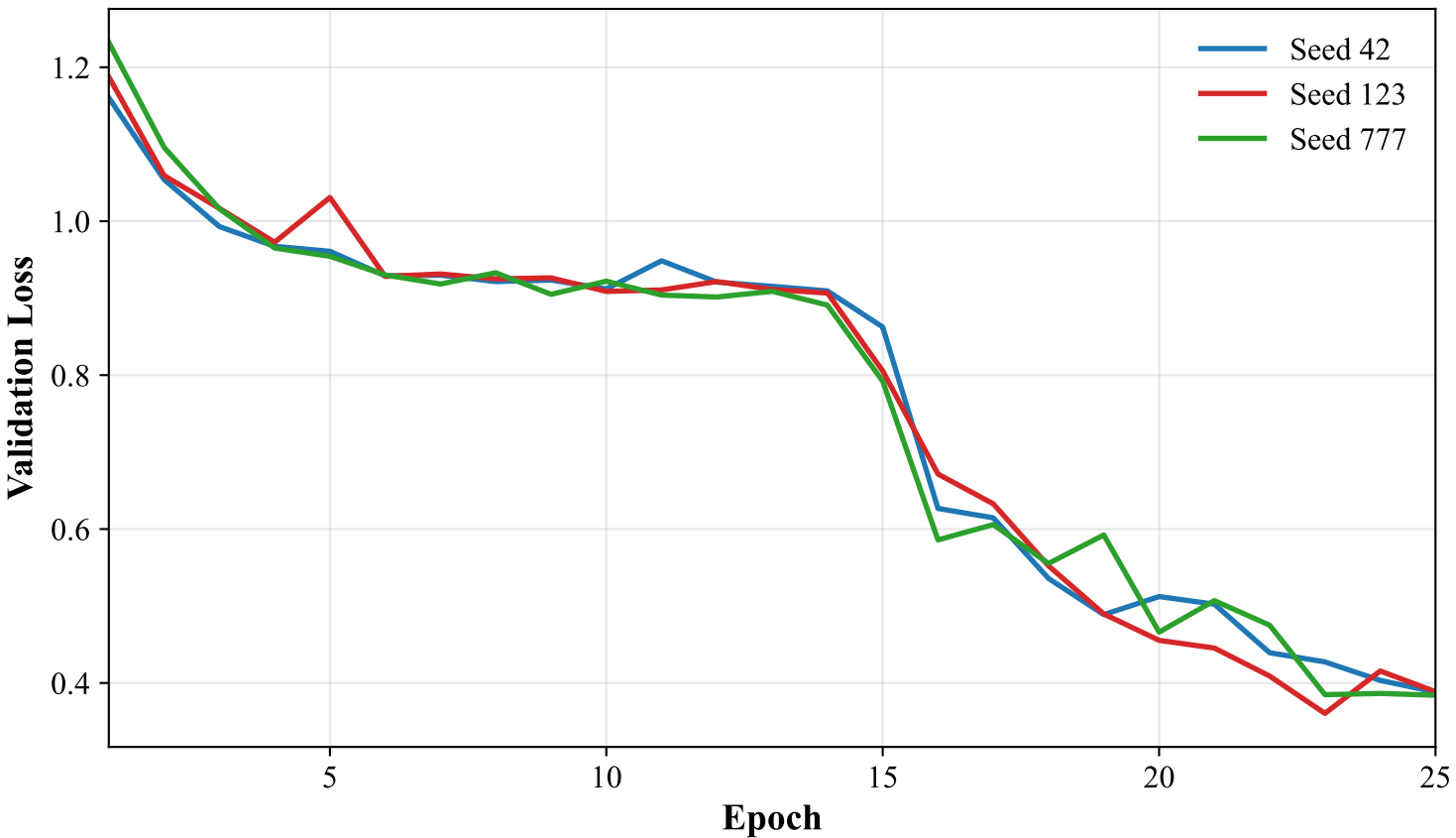
ERP-CBAM Validation Loss Across Random Seeds
